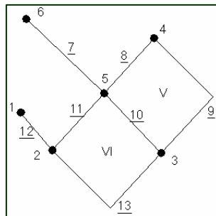
Macierz S_{P-K}
